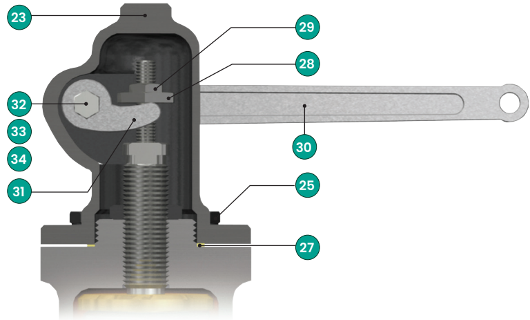
Packed Lever
