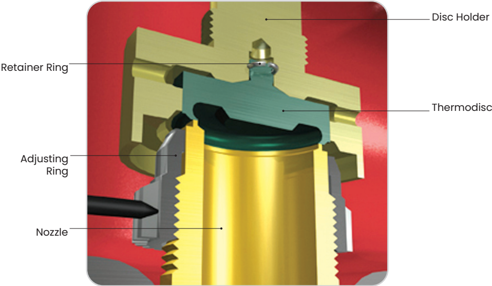
Steam Trim Internals
