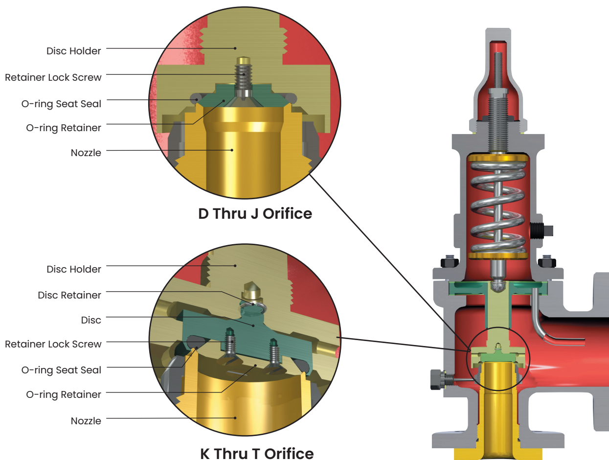
Standard Material for 1900/1900 DM Soft Seat (DA) Safety Relief Valves
