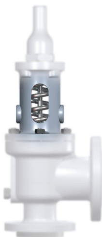
Slotted Bonnet
